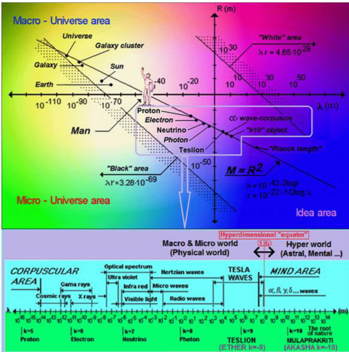
Fig. 1, "Energy-space" diagram
